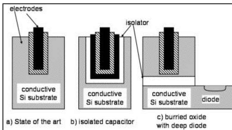
Figure 24-2: Trench capacitors
