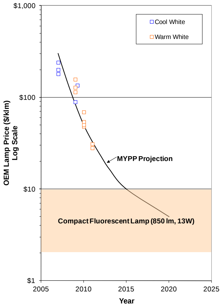
Figure 3.4: White Light Integrated LED Lamp Price Projection (Logarithmic Scale) Note: Assumes current prices for compact fluorescent price range (13W self-ballasted compact fluorescent; non-dimmable at bottom, and dimmable at top).
